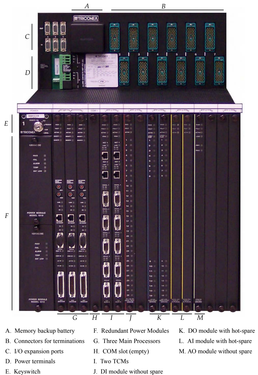
Sample Layout of a Tricon Chassis
