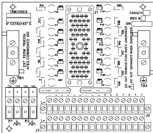
16-Point Nonincendive Digital Output Termination Panels
