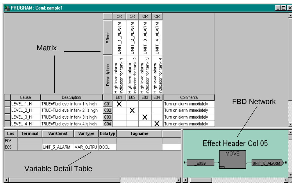
CEM Editor Components
