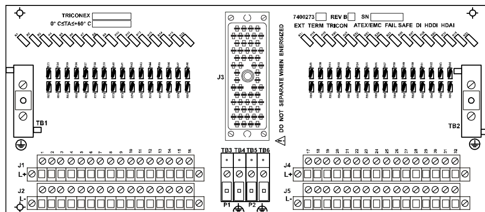
32-Point Nonincendive Analog Input and Digital Input Termination Panels
